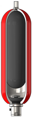
Bladder Accumulator* 1PT - 40 GAL 3000 to 10000 PSI (Top Repairable Design Available for 3000 & 6000 PSI)
